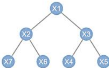
XGBoost
