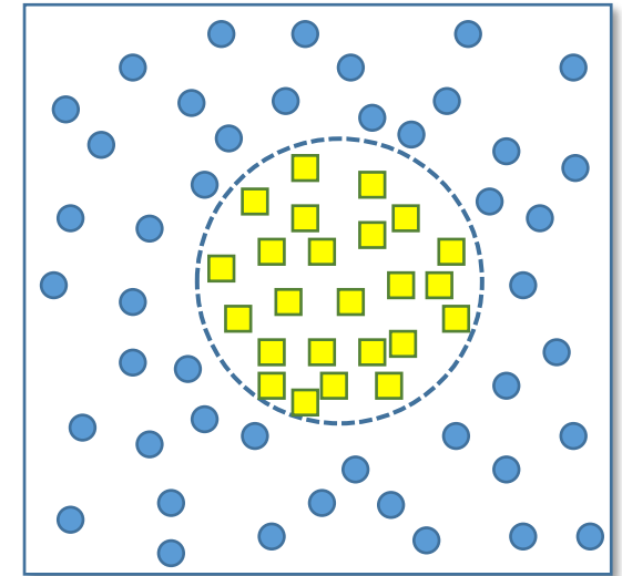
Case 3
